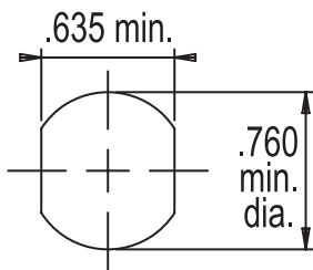
Mounting hole
