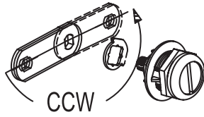
RH DRAWER
