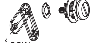
DRAWER
