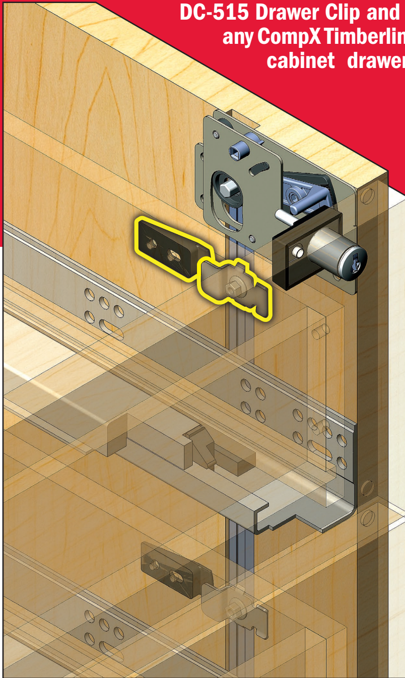
SHOWN IN LOCKED POSITION
